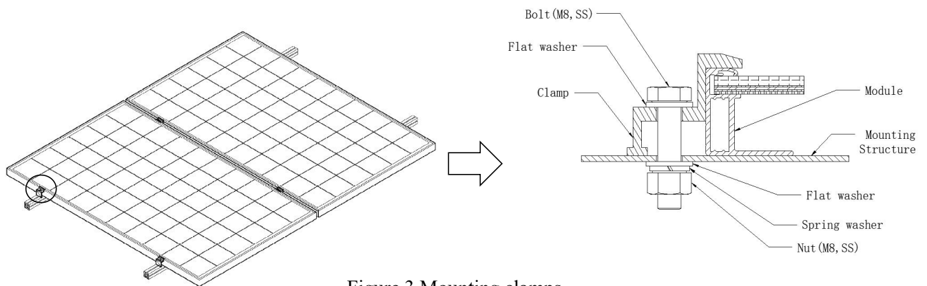
Figure 3 Mounting clamps
